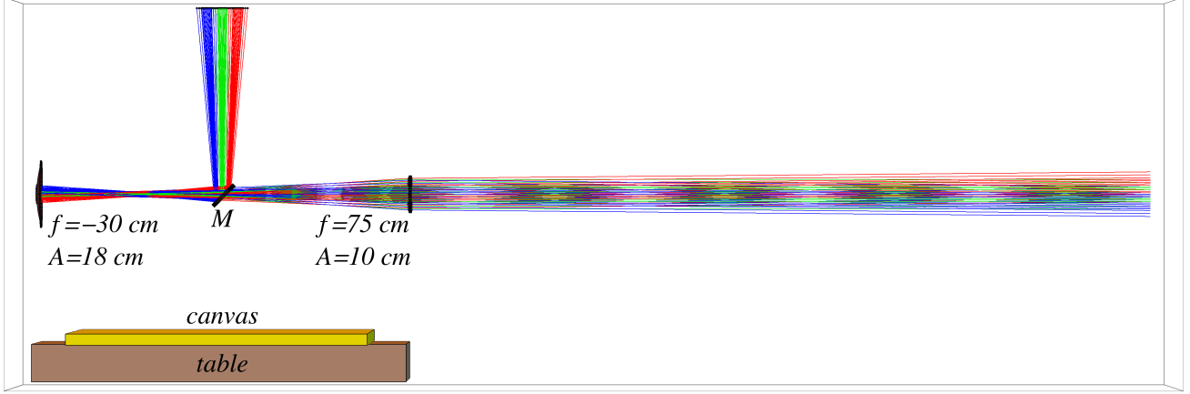
Figure 1. Ray-tracing diagram of Jenison’s final optical telescope and mirror comparator used for copying/transcribing the studio reconstruction of Vermeer’s Lady at the virginals with a gentleman . [21, 34:01] The studio is off to the right and light passes from it through a converging lens (focal length f = 75\text{ cm} , aperture diameter A = 10\text{ cm} ), then to a concave mirror ( f = -30\text{ cm} , A = 18\text{ cm} ) back to a small plane “secondary mirror,” M , then up to the artist’s eye. The focal lengths, aperture diameters, and rough separations of components were taken from a diagram from Jenison’s notebooks. The colored rays correspond to distant points on the optical axis and at \pm 0.5^\circ . The artist/copyist could look down at the plane secondary mirror, M , to see the real image of the tableau, then shift slightly to the side to see the corresponding position on the canvas where he had applied paint. In this way, the artist/copyist could adjust the applied paint until the two images matched.
